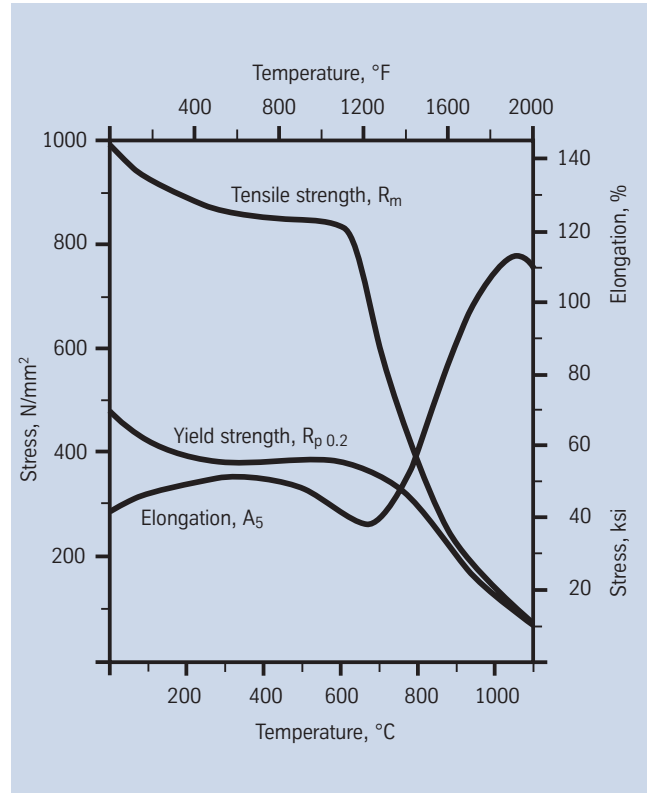
Fig. 1 – Typical short-time mechanical properties at elevated temperatures of cold rolled, Nicrofer 6020 hMo annealed at 1000 °C (1830 °F).
