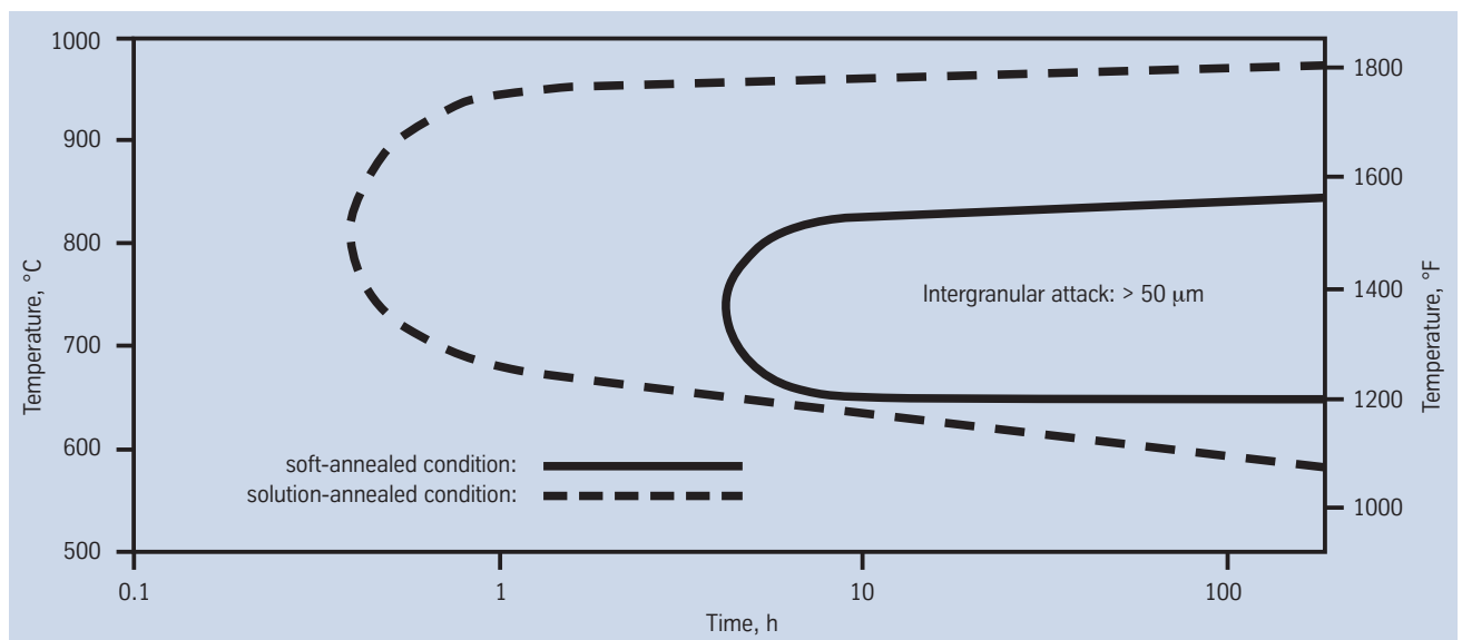
Fig. 2 – Time-Temperature-Sensitization (TTS) diagram for Nicrofer 6020 hMo (0.02 % carbon) according to ASTM G-28 A, (120 h).
